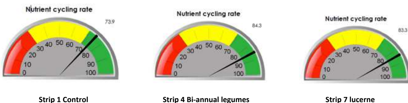
Figure 17 Soil biology indicator diagrams indicating nutrient cycling rate
